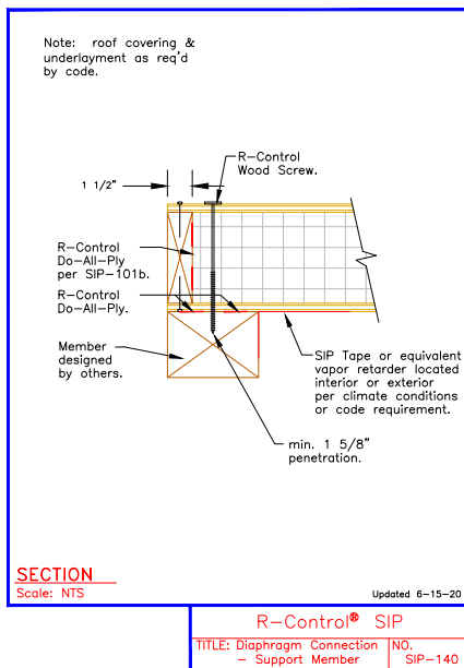
R-Control® SIP TITLE: Diaphragm Connection - Splines NO. SIP-139a
